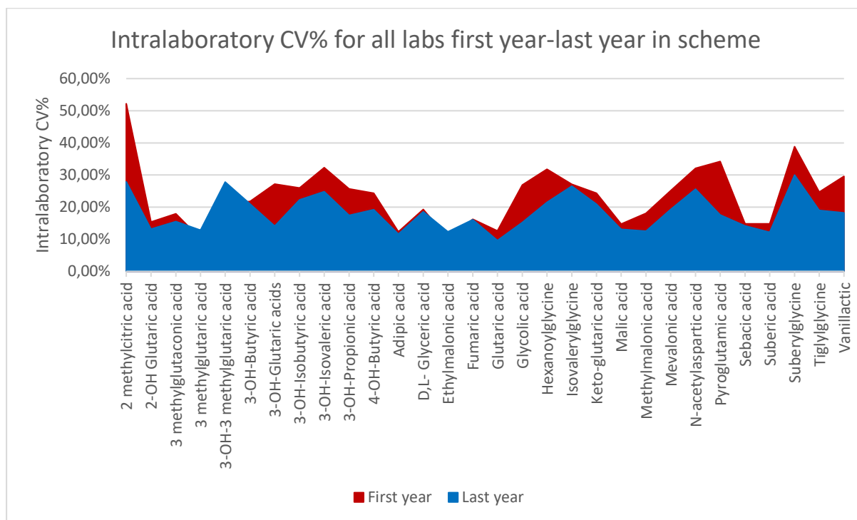
Figure 1: Difference in Intralaboratory CV% of all labs between the first year and the last year of compound introduction in scheme
