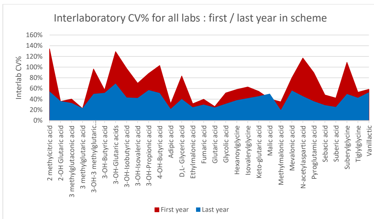
Figure 2: Difference in Interlaboratory CV% of all labs between the first year and the last year of compound introduction in scheme
